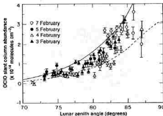
Fig. 3. Observations of the increase in OCIO slant column abundance as a function of increasing lunar zenith angle for all moonset data obtained at Thule in February 1988. See Table 1 for background spectra used on each night. Lines indicate the expected response for OCIO vertical column abundances of (---) 3 \times 10^{13} and (—) 6 \times 10^{13} \text{ molecules cm}^{-2} . The background lunar zenith angle was approximately 65^\circ to 70^\circ .
