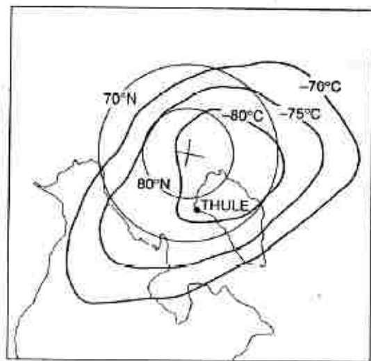
Fig. 1. National Meteorological Center (NMC) 30-mbar (~24-km altitude) temperature analysis 4 February 1988.
