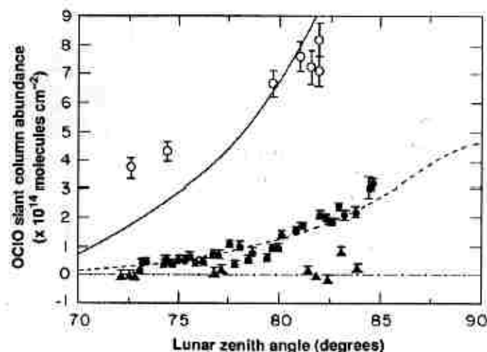
Fig. 2. Observations of the increase in OCIO slant column abundance as a function of increasing lunar zenith angle at Fritz Peak, Colorado ( \blacktriangle , 40°N), on 3 January 1988, at Thule, Greenland ( \bullet , 76.5°N), on 3 February 1988, and at McMurdo Station, Antarctica ( \circ , 78°S), on 30 August 1987. The background spectrum used in the analysis in all cases was taken near 65° lunar zenith angle on the indicated nights. Lines indicate the expected response for OCIO vertical column abundances of (—) 0, (---) 4.5 \times 10^{13} , and (—) 2.5 \times 10^{14} molecules cm -2 .
