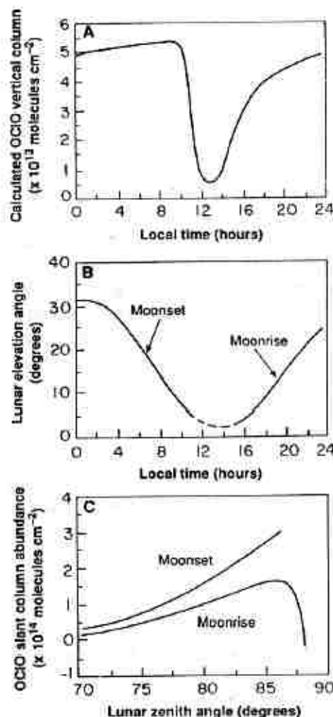
Fig. 4. (A) Calculated diurnal variation of the OCIO vertical column abundance obtained by multiplying the reactive chlorine abundances of the model by Garcia and Solomon (26) by a factor of 10 (see text). (B) Lunar elevation angle as a function of local time on the night of 3-4 February 1988 at Thule, Greenland. (C) Calculated variation of OCIO slant column abundance versus lunar zenith angle based on that in (A) and (B), assuming a background lunar zenith angle of 65^\circ .
